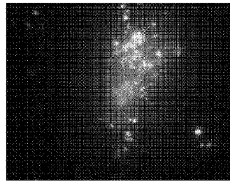
beta-D-thio-LNA; 2746
