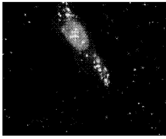
beta-D-oxy-LNA; 2740
