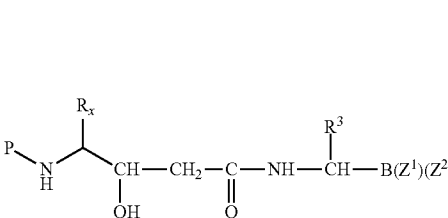
statine alalog
