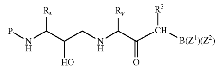
hydroxyethylamine isostere
