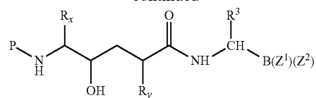
hydroxyethylene isostere
