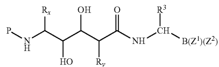
dihydroxyethylene isostere
