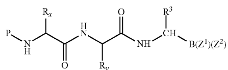
peptide bond
