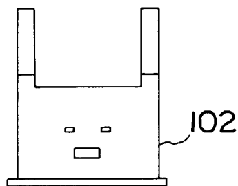
FIG. 32 PRIOR ART
