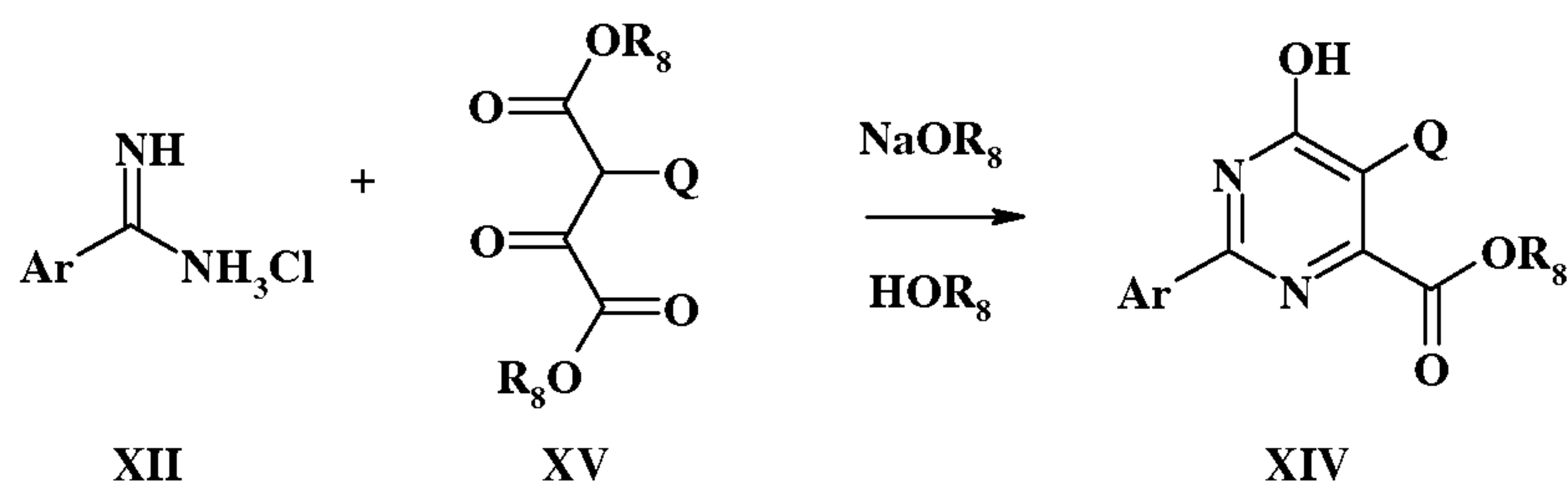
Scheme 7
