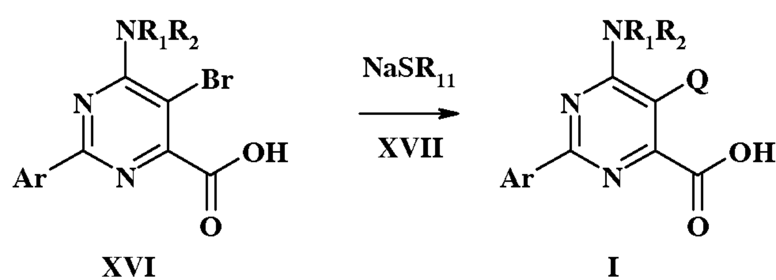
Scheme 8
