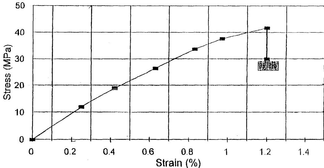
Typical stress - strain behavior Natural fiber composite
