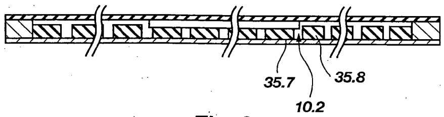
Fig. 3 (PRIOR ART)
