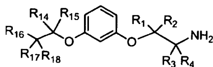
Formula (IIb)
