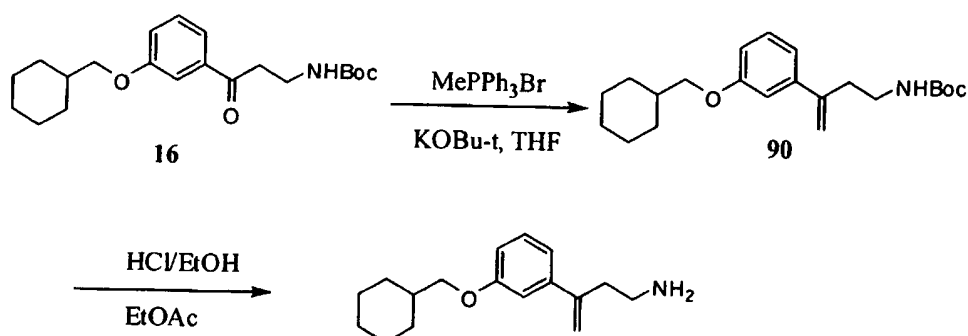
SCHEME 27
