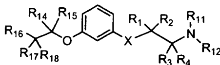
Formula (II)
