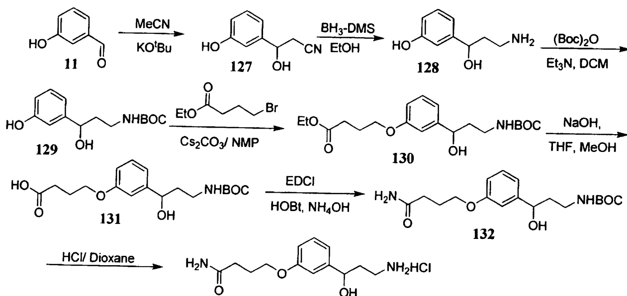
SCHEME 42
