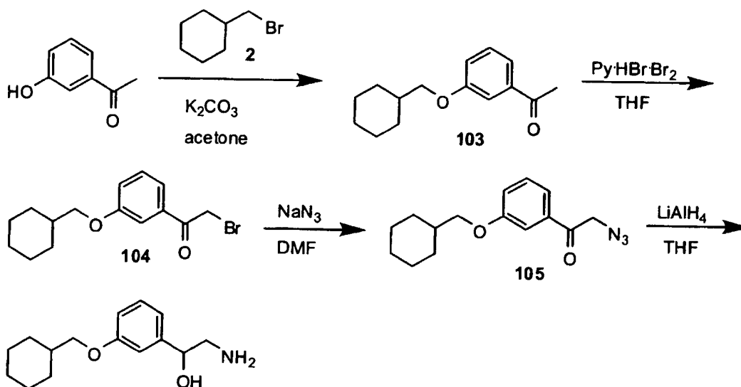
SCHEME 35
