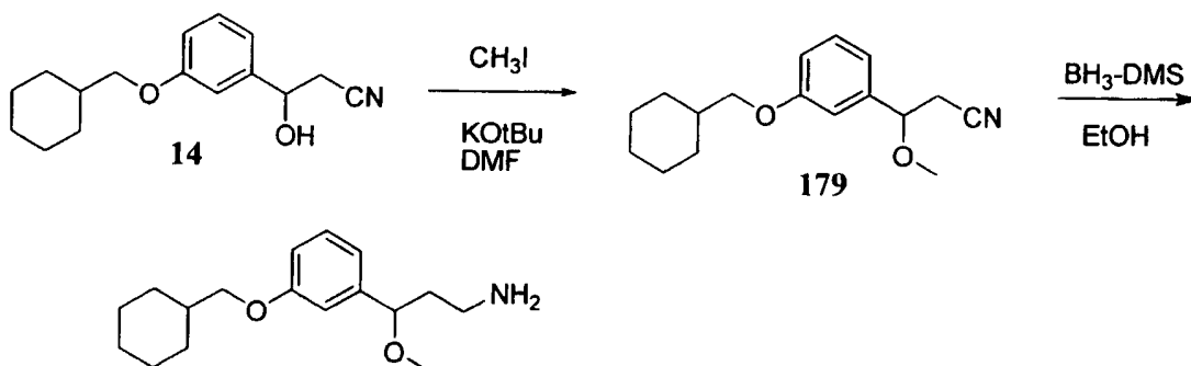
SCHEME 57
