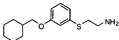
SCHEME 31
