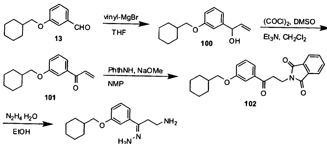
SCHEME 34
