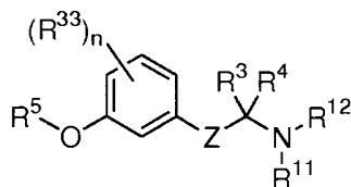
Formula (A)
