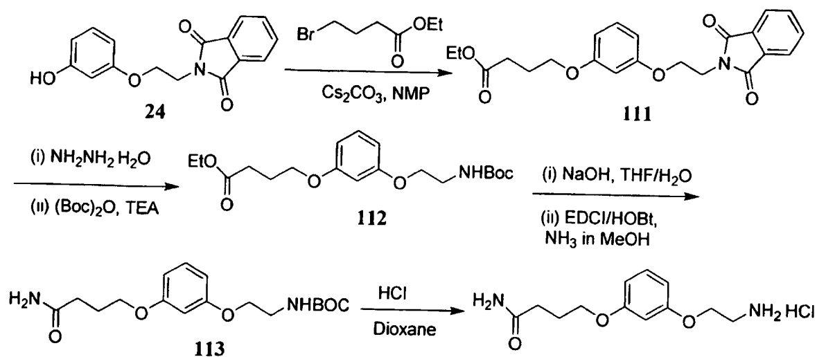
SCHEME 38
