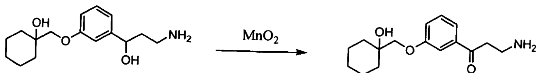
SCHEME 13
