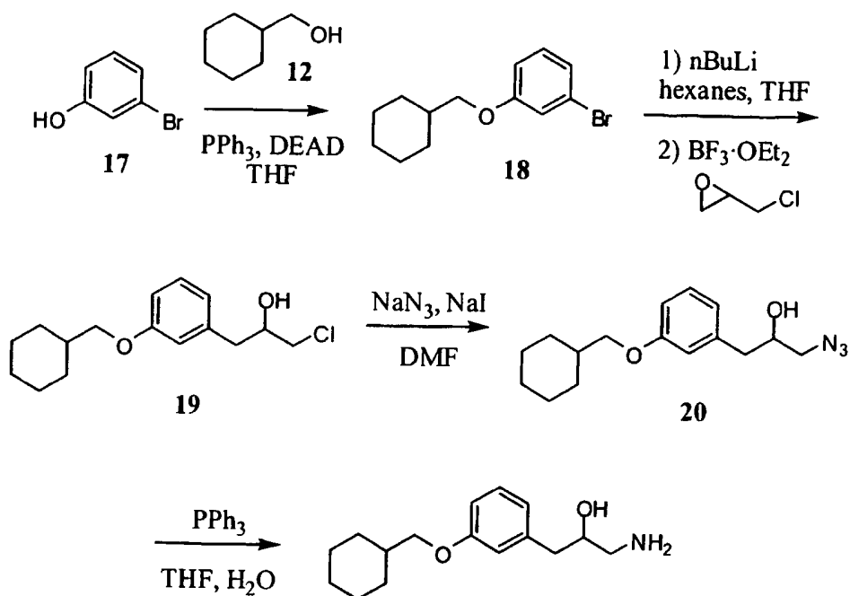
SCHEME 5
