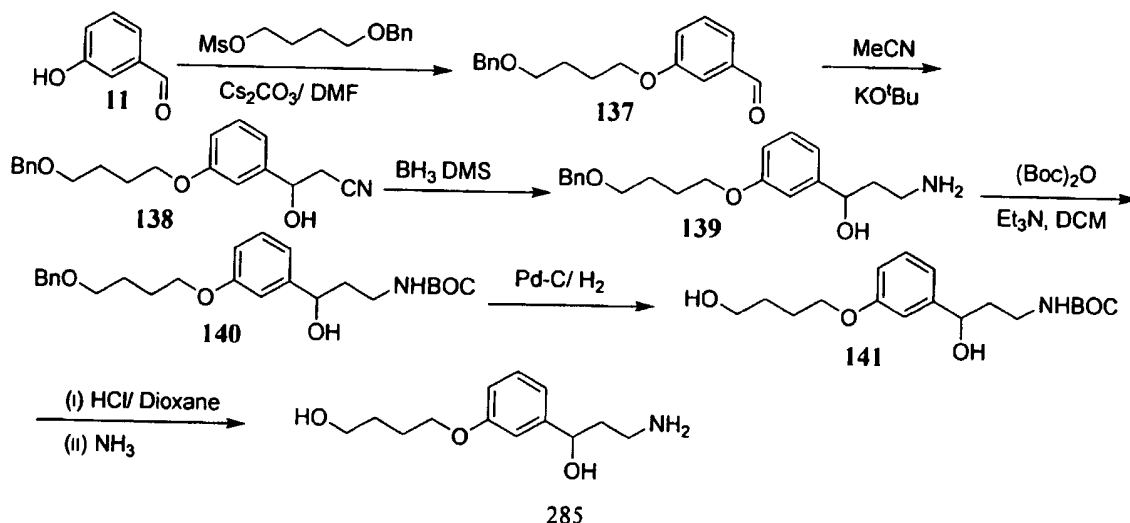
SCHEME 45
