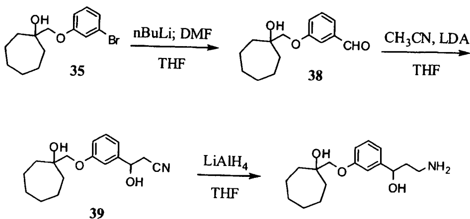
SCHEME 9
