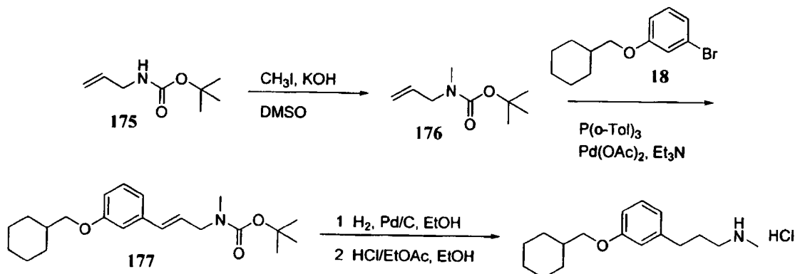
SCHEME 54
