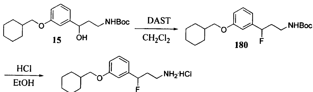
SCHEME 58
