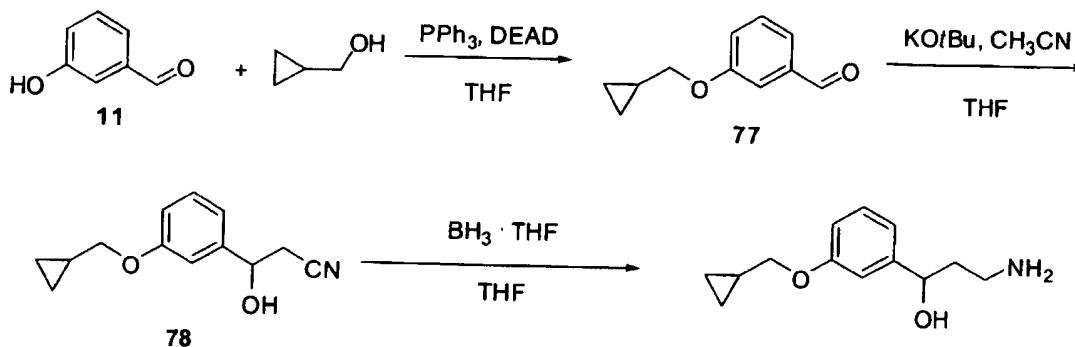
SCHEME 22
