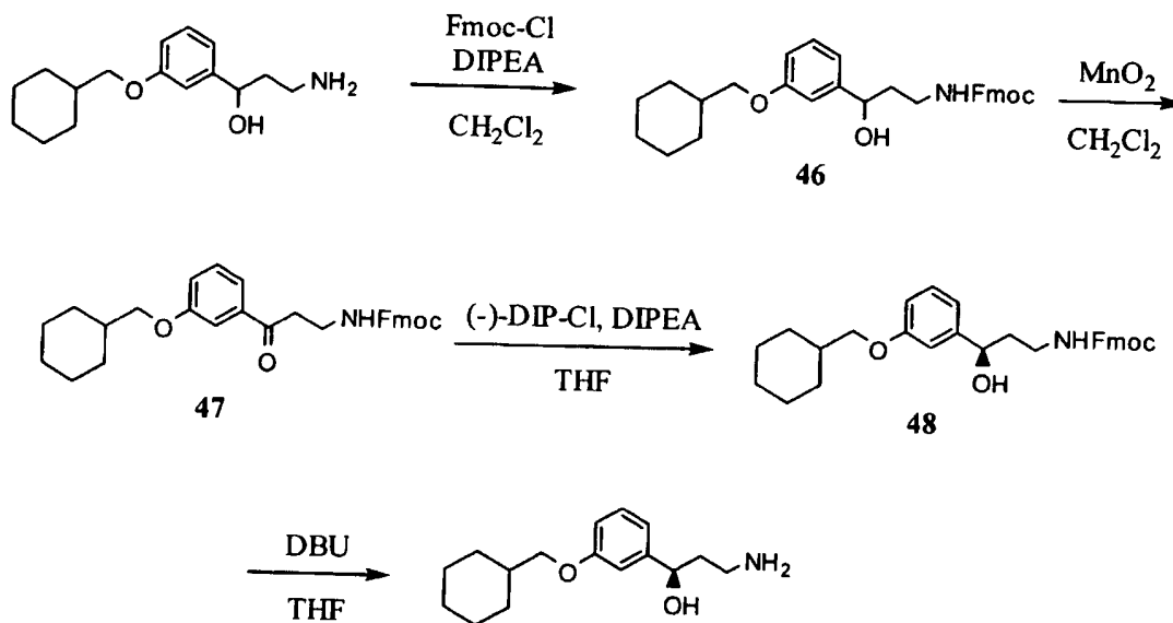
SCHEME 14
