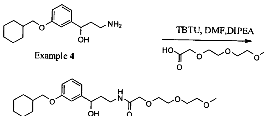
SCHEME 26
