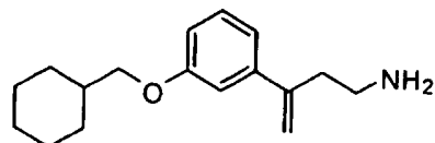
SCHEME 27
