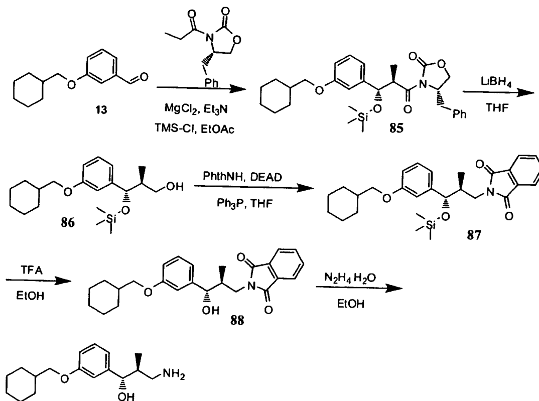
SCHEME 24
