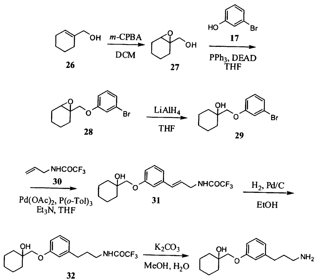
SCHEME 7
