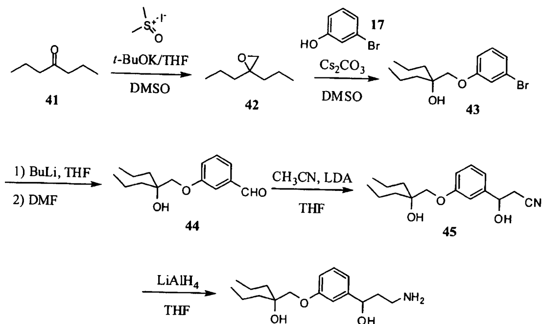
SCHEME 12
