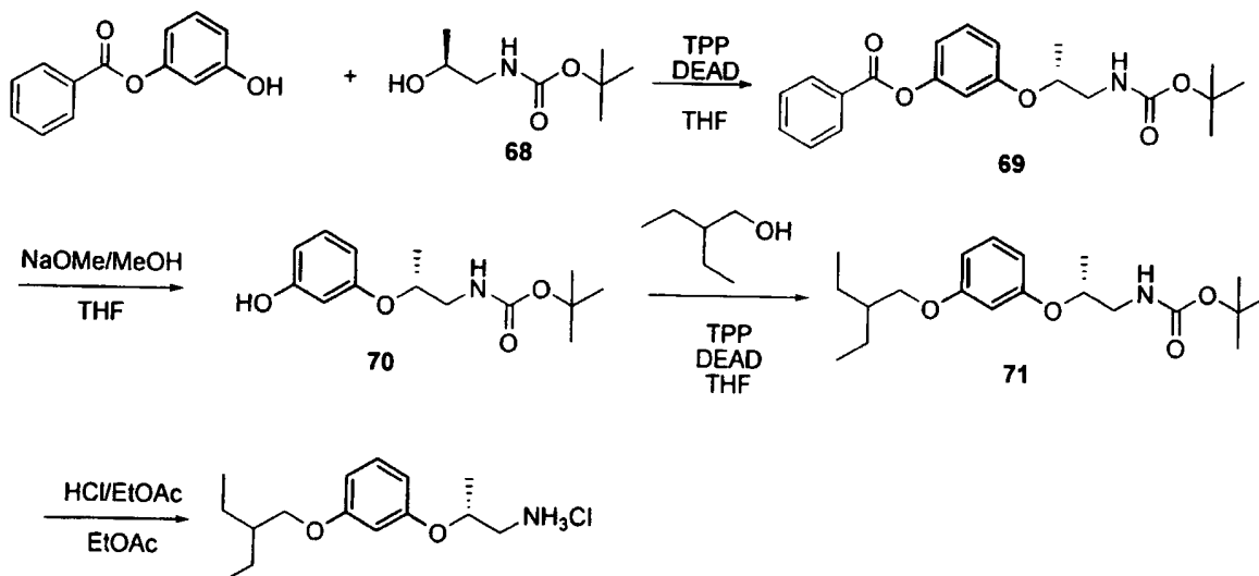
SCHEME 20
