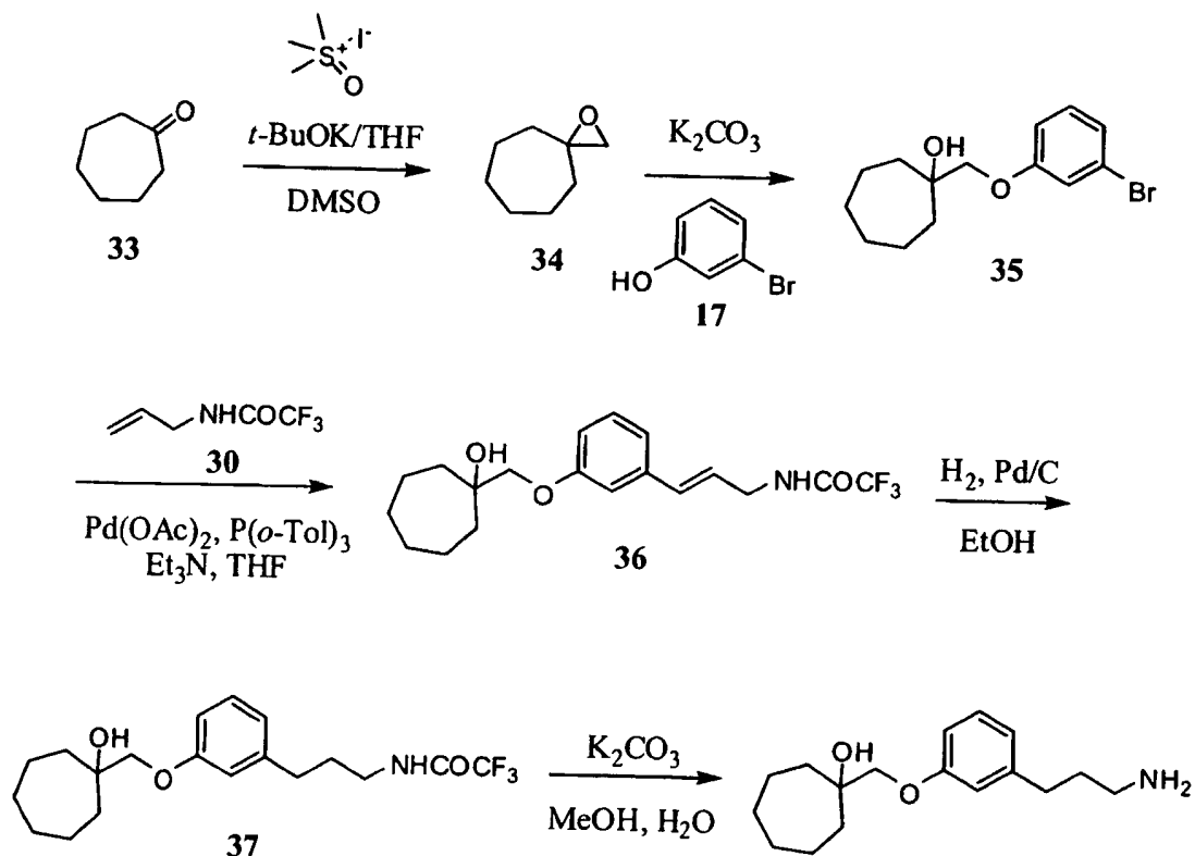
SCHEME 8
