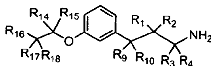
Formula (IIa)
