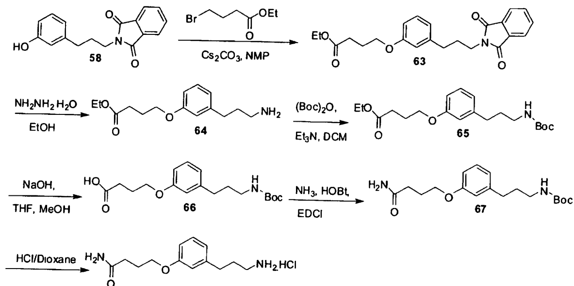
SCHEME 19
