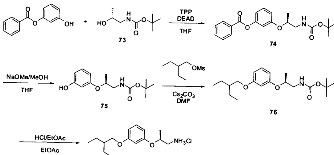
SCHEME 21
