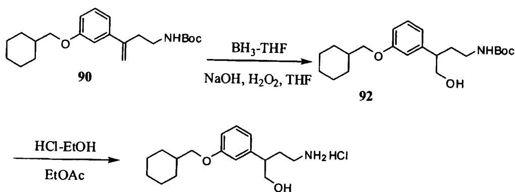
SCHEME 29
