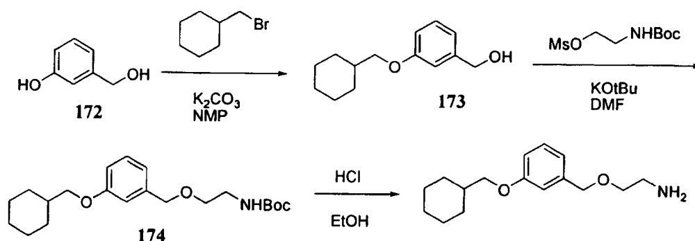
SCHEME 53
