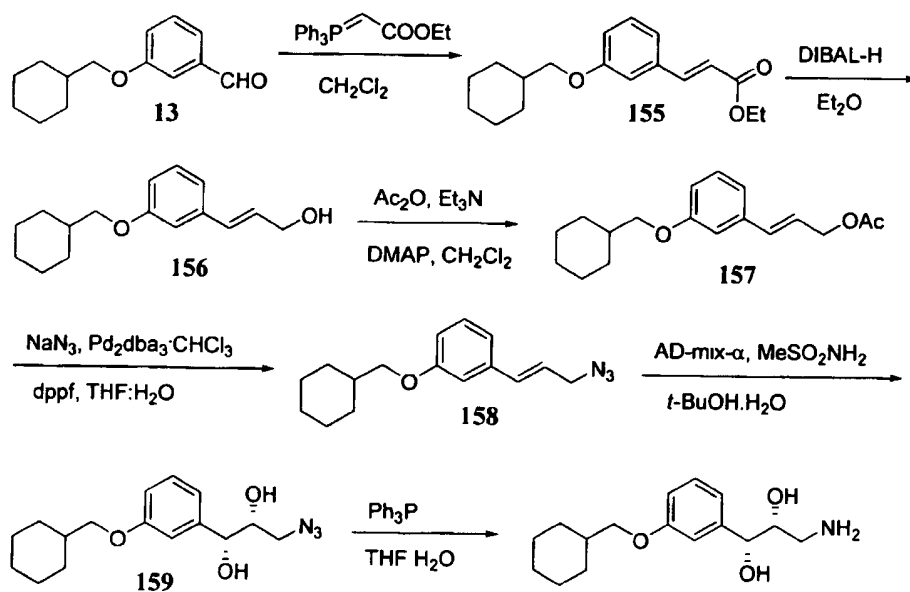
SCHEME 49
