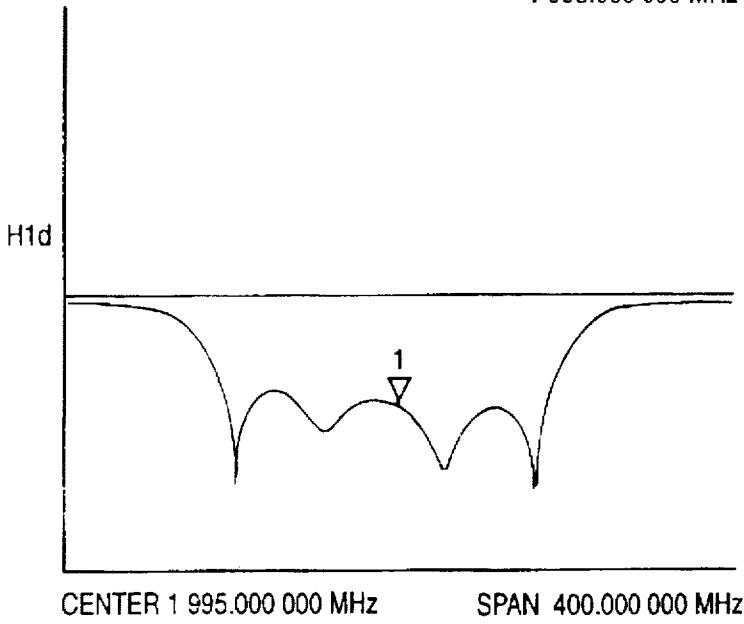
FILTER RETURN LOSS
