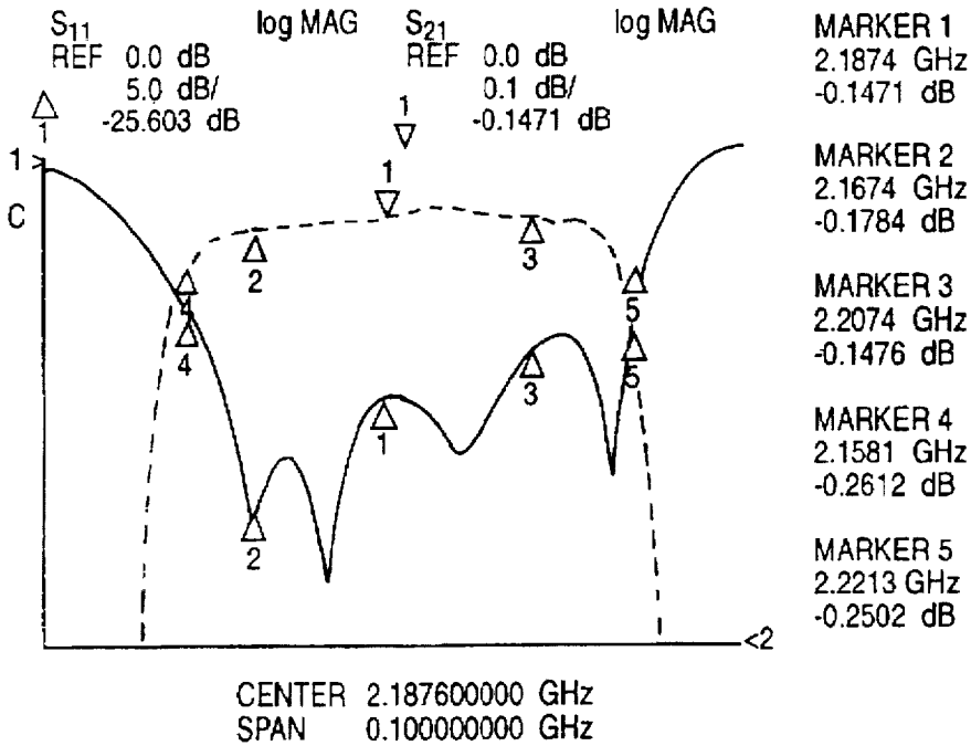
FILTER PASSBAND AND RETURN LOSS
