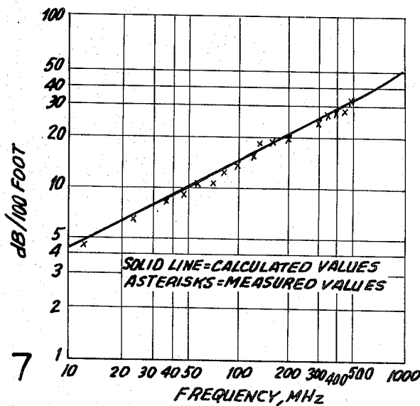
SINE WAVE ATTENUATION OF PROTOTYPE CABLE (CA-490)
