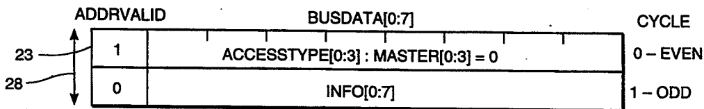
FIG 5 REJECT (NACK) CONTROL PACKET
