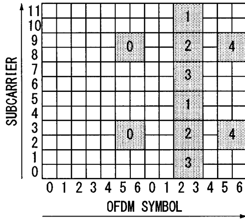
(c) 8 CSI-RS PORTS
