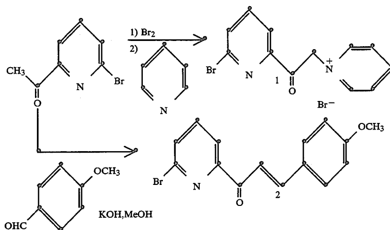
Reaction Scheme I Synthesis of THT and TMT
