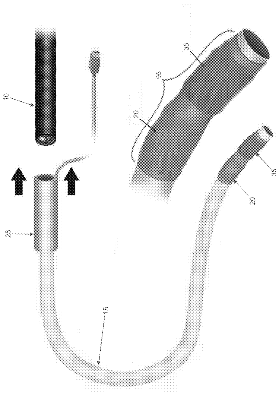
2. Pull disposable device over scope then remove condom from tip of scope
