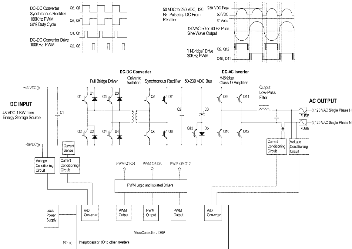
BIDIRECTIONAL INVERTER: AC GENERATION MODE FUNCTIONAL BLOCK DIAGRAM
