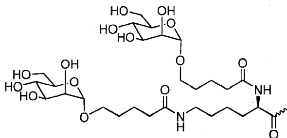
Formula XXII.
