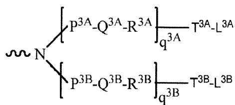
Formula XXXIII
