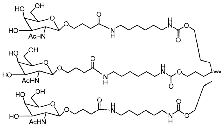
Formula IX,
