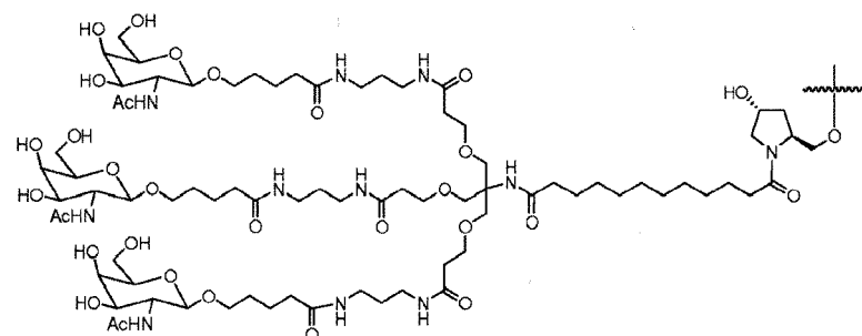
(Formula XXV),
