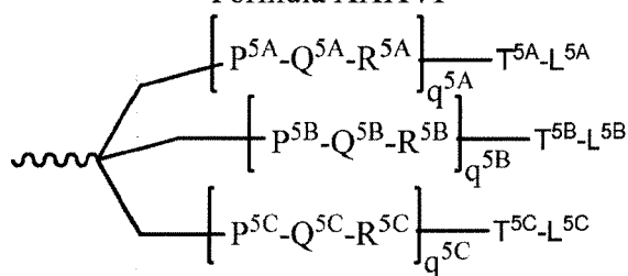
Formula XXXVI
