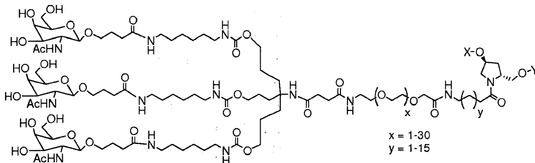
(Formula XXVII),
