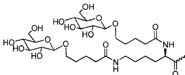
Formula XVIII,
