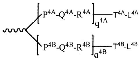
Formula XXXIV
