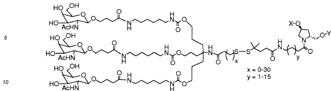
(Formula XXVIII),
