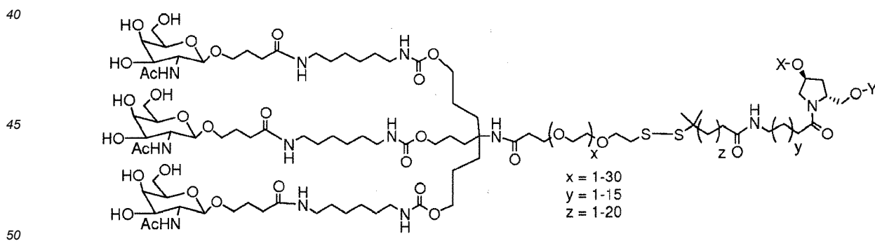
(Formula XXXI),
