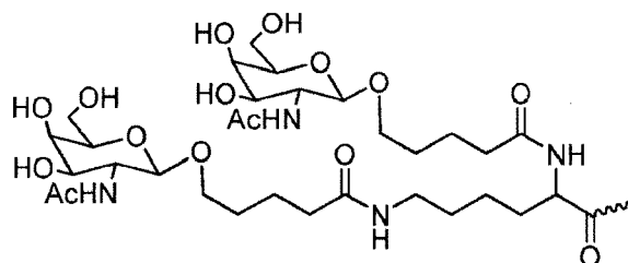
Formula XVI,
