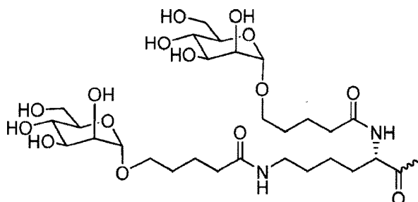
Formula XXI,
