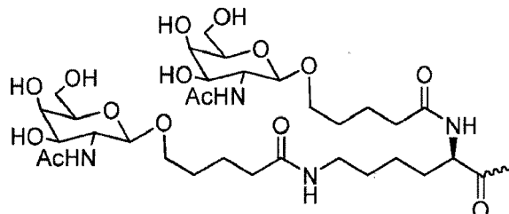
Formula XV,
