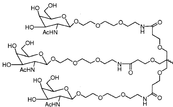
Formula X,
