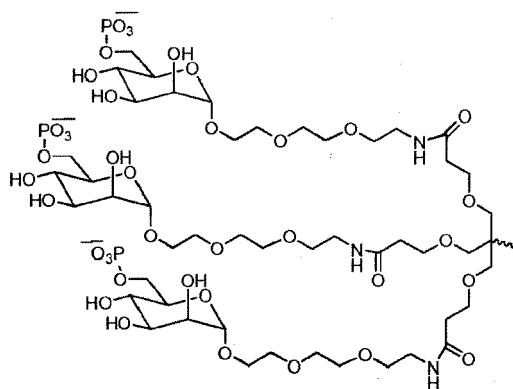
Formula XI,
