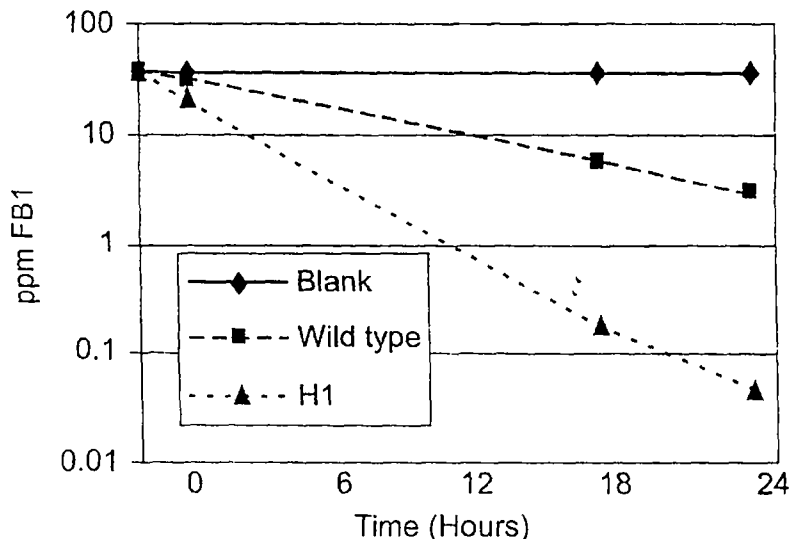
H1 reduces FB1 below 0.1 ppm in 24 hrs Time course of FB1 degradation (pH 5.5)
