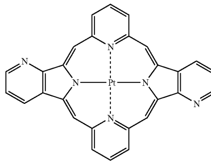
Compound (29)
