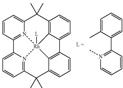
Compound (122)
