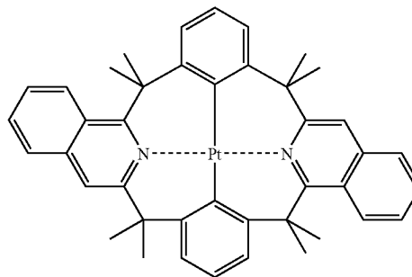
Compound (148)
