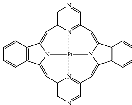
Compound (28)
