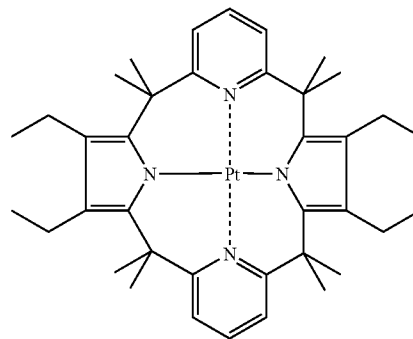
Compound (141)
