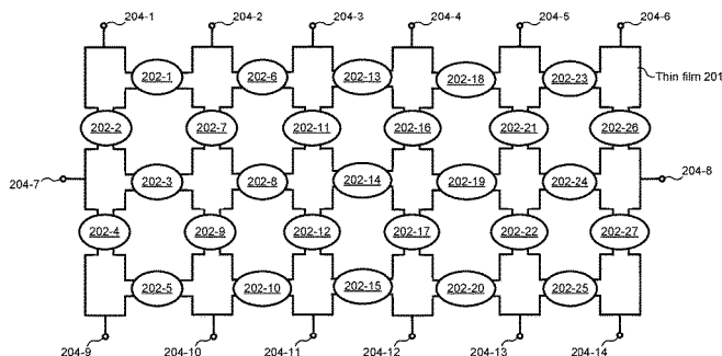
Superconducting Circuit 200
