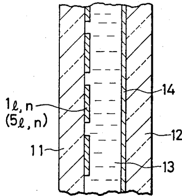
FIG. 1 PRIOR ART
