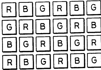
FIG. 3 PRIOR ART
