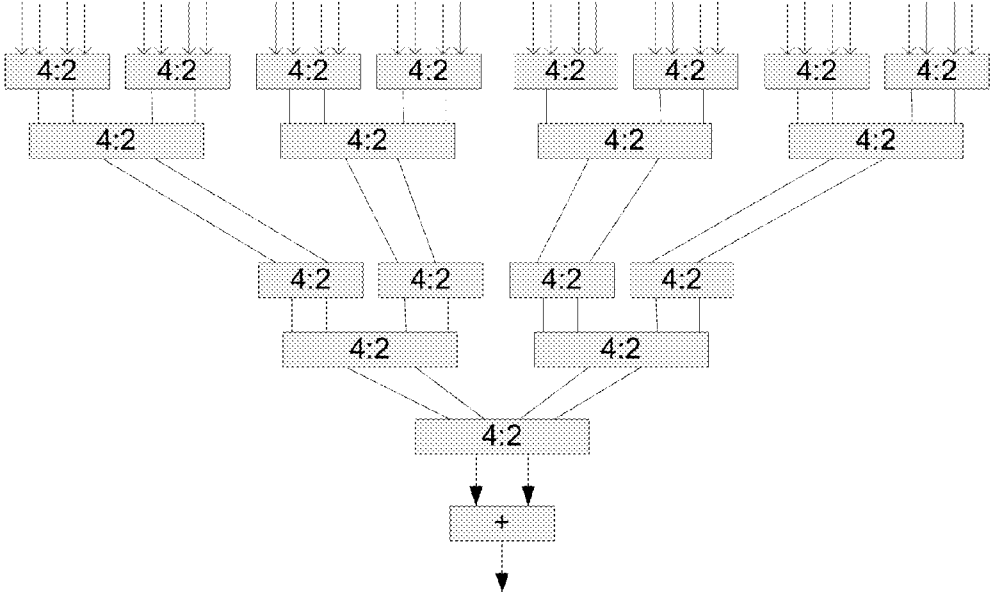
Carry save adder parallel implementation of an exemplary adder (x)
