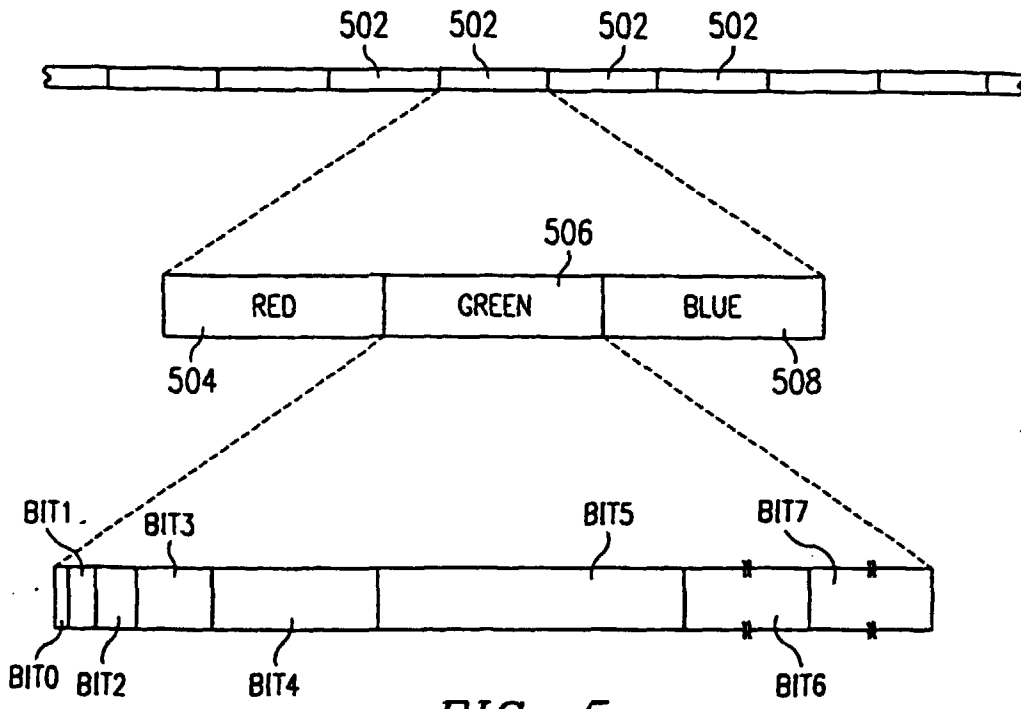
FIG. 5 (PRIOR ART)
