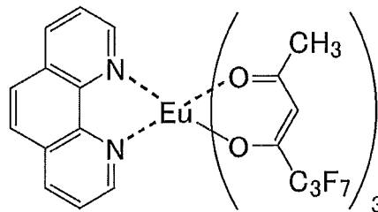
[Eu(FPD) 3 ]phen
