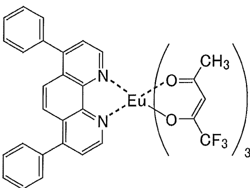
Eu(TFA) 3 dpphen
