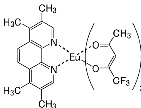
[Eu(TFA) 3 ]tmphen
