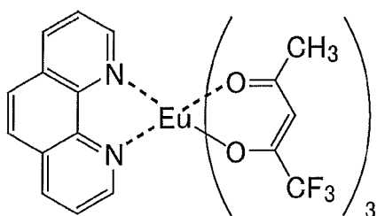
Eu(TFA) 3 phen
