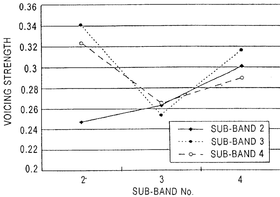
2ND, 3RD, 4TH SUB-BAND VOICING STRENGTH (FOR UNVOICED STATE)
