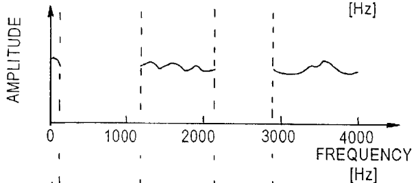
FIG. 6E OUTPUT (r8) OF NOISE EXCITATION FILTERING UNIT
