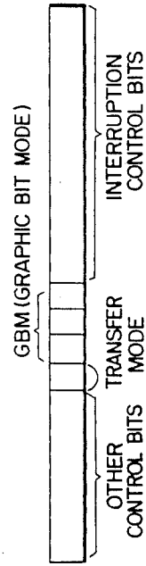
FIG. 8f INSTRUCTION CONTROL REGISTER (230)
