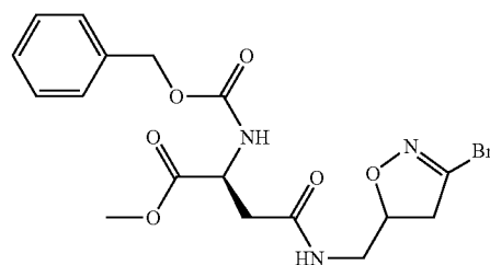
(S)-2-Benzyloxycarbonylamino-N-(3-bromo-4,5-dihydro-isoxazol-5-ylmethyl)-succinamic acid methyl ester
