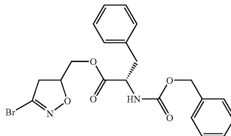
(S)-2-Benzyloxycarbonylamino-3-phenyl-propionic acid 3-bromo-4,5-dihydro-isoxazol-5-ylmethyl ester
