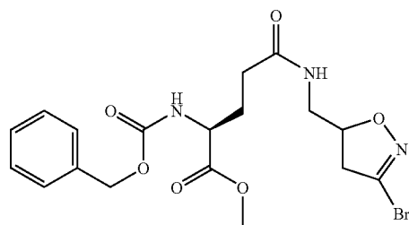
(S)-2-Benzyloxycarbonylamino-4-[(3-bromo-4,5-dihydro-isoxazol-5-ylmethyl)-carbamoyl]-butyric acid methyl ester
