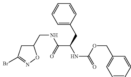
((R)-1-[(3-Bromo-4,5-dihydro-isoxazol-5-ylmethyl)-carbamoyl]-2-phenyl-ethyl)-carbamic acid benzyl ester
