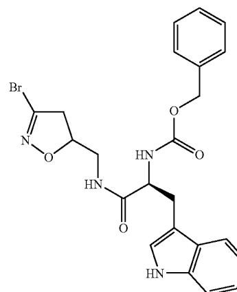
((S)-1-[(3-Bromo-4,5-dihydro-isoxazol-5-ylmethyl)-carbamoyl]-2-(1H-indol-3-yl)-ethyl)-carbamic acid benzyl ester
