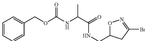
((S)-1-[(3-Bromo-4,5-dihydro-isoxazol-5-ylmethyl)-carbamoyl]-ethyl)-carbamic acid benzyl ester
