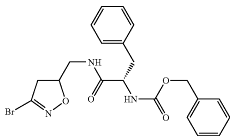
{(S)-1-[(3-Bromo-4,5-dihydro-isoxazol-5-ylmethyl)-carbamoyl]-2-phenyl-ethyl)-carbamic acid benzyl ester
