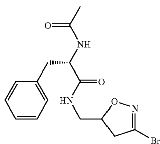
(S)-2-Acetylamino-N-(3-bromo-4,5-dihydro-isoxazol-5-ylmethyl)-3-phenyl-propionamide
