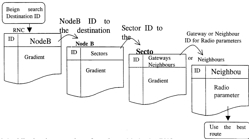
Linked list implementation of routing table in the RNC
