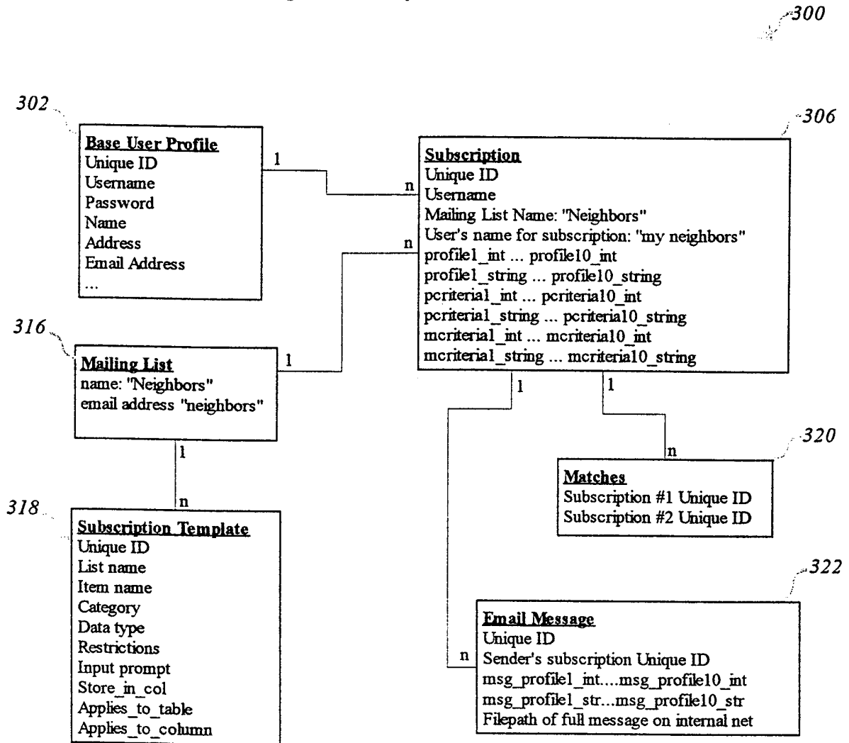
Figure 3a: System's Database
