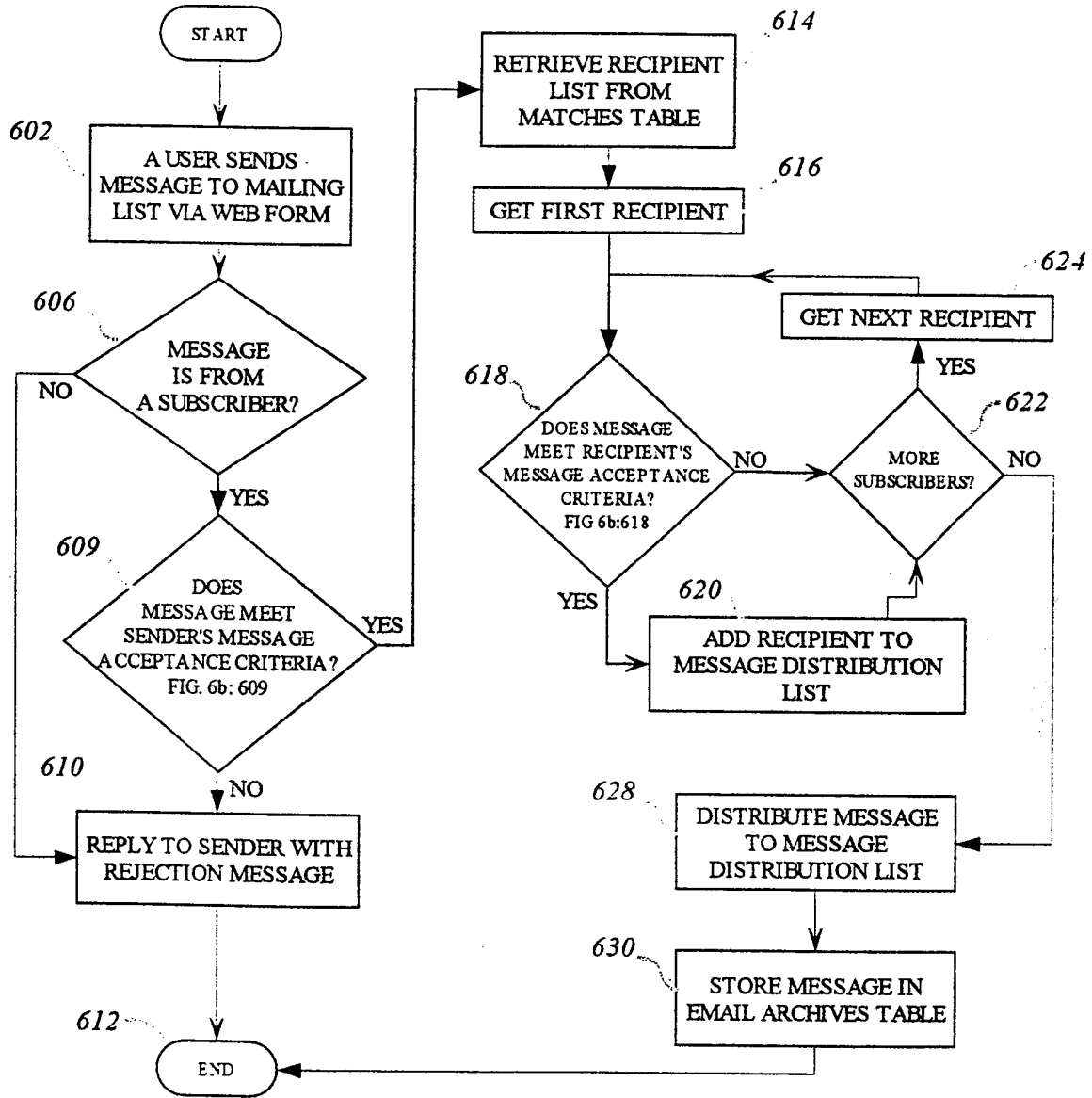
Figure 6a: Message Distribution Process
