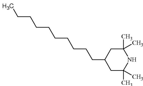
2,2,6,6-tetramethyl-4-butylpiperidine:
