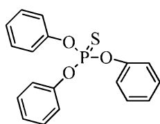
Triphenyl Phosphorothionate
