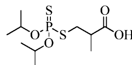
Acidic Dialkyl Dithiophosphate
