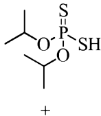
Neutral Dialkyl Dithiophosphate
