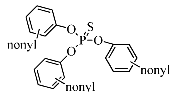
Nonyl Triphenyl Phosphorothionate
