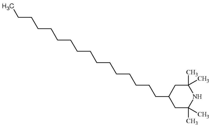
2,2,6,6-tetramethyl-4-hexadecylpiperidine:
