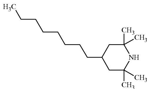
2,2,6,6-tetramethyl-4-decylpiperidine:
