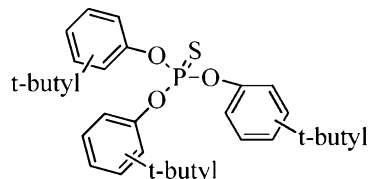
Butylated Triphenyl Phosphorothionate
