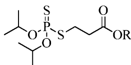
Neutral Dialkyl Dithiophosphate
