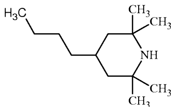
2,2,6,6-tetramethyl-4-hexadecylpiperidine:
