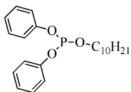
Decyl Diphenylphosphite
