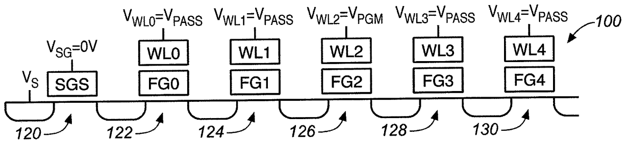
FIG. 4C (PRIOR ART)
