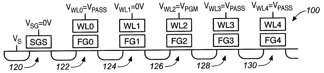
FIG. 6C (PRIOR ART)
