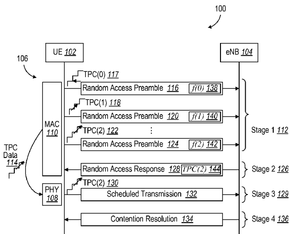
Contention-Based Random Access (RACH) Procedure
