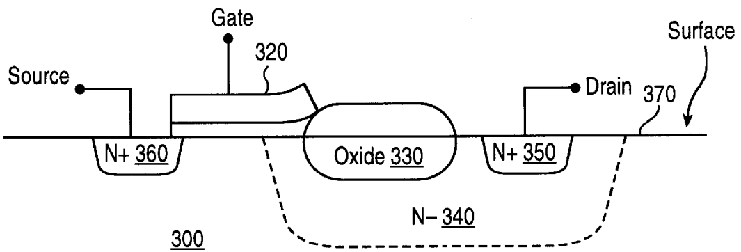
Vertical drain N-Channel metal-oxide semiconductor (VDNMOS) transistor
