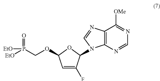
(2'R,5'R)-6-Methoxy-9-[3-fluoro-2,5-dihydro-5-(diethoxyphosphinyl)methoxy-2-furanyl]purine (7)
