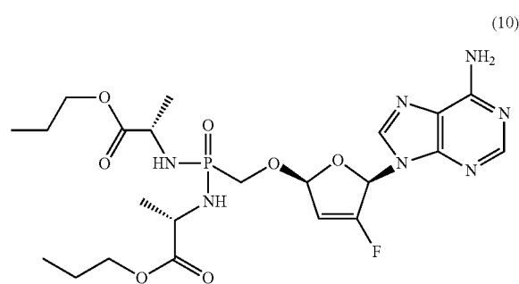
Example of Bis Amidate Preparation (10)
