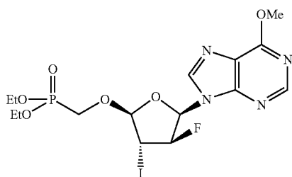
(2'R,3'S,4'R,5'R)-6-Methoxy-9-[tetrahydro 4-iodo-3-fluoro-5-(diethoxyphosphinyl)methoxy-2-furanyl]purine (6)
