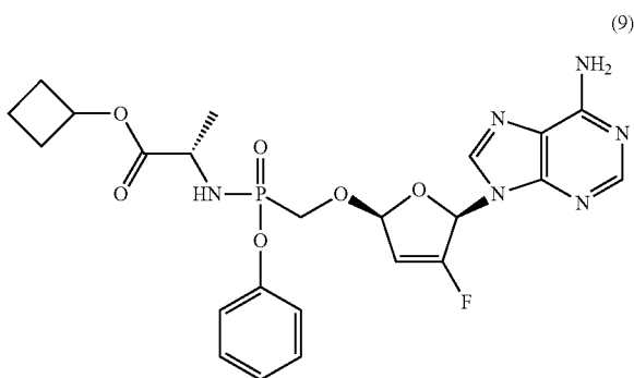
Example of Monoamidate Preparation (9)
