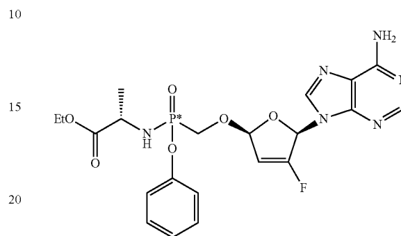
Example of Monoamidate Preparation (11)
