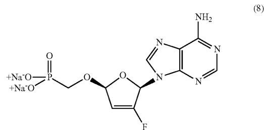
(2'R,5'R)-9-(3-fluoro-2,5-dihydro-5-phosphonomethoxy-2-furanyl)adenine di sodium salt (8)
