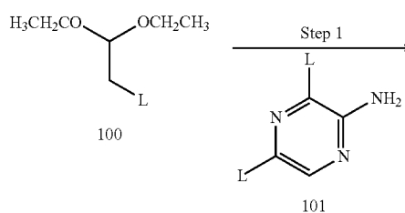
Reaction Scheme 1
