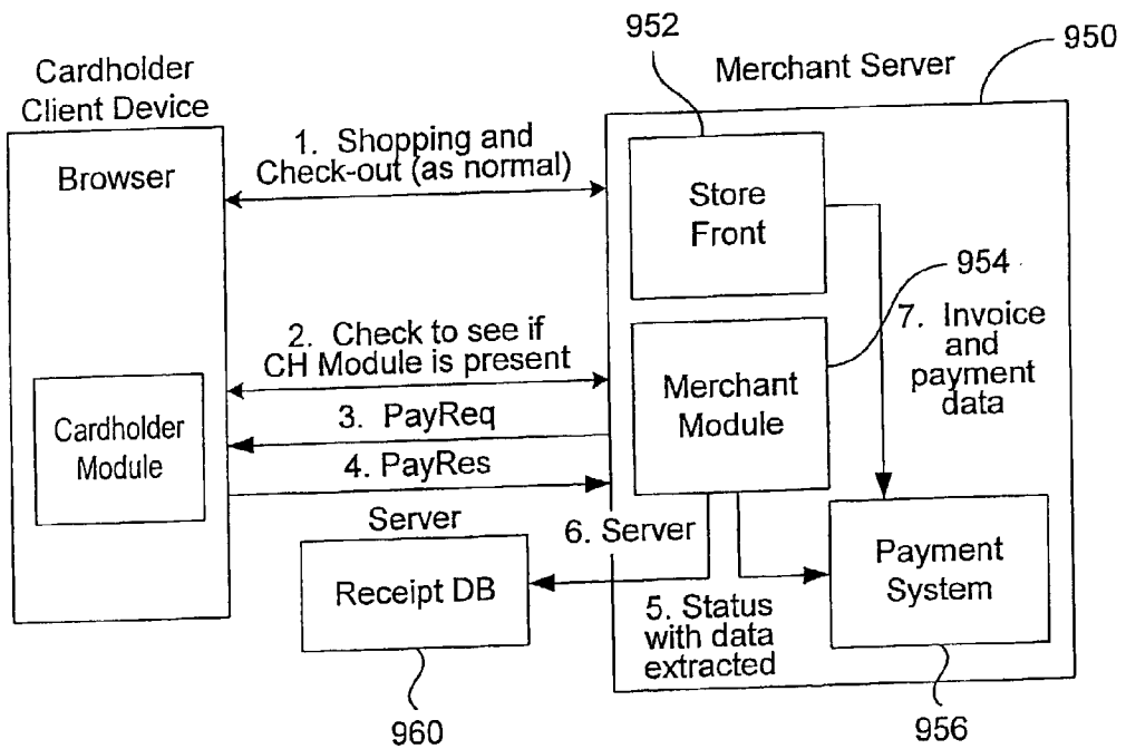
FIG. 10 Distributed Payment Flow
