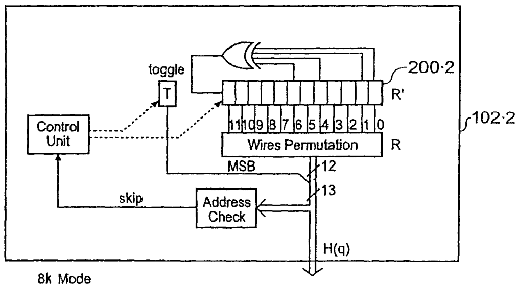
Fig. 6 BACKGROUND ART
