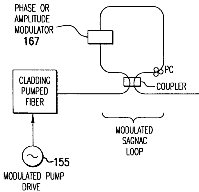
FIG. 14c PRIOR ART
