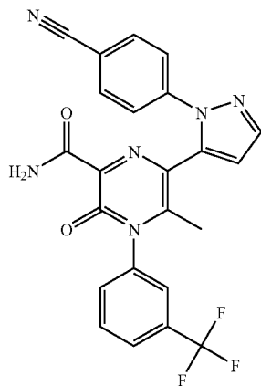
6-[1-(4-Cyanophenyl)-1H-pyrazol-5-yl]-5-methyl-3-oxo-4-[3-(trifluoromethyl)phenyl]-3,4-dihydropyrazine-2-carboxamide
