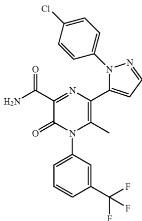
6-[1-(4-Chlorophenyl)-1H-pyrazol-5-yl]-5-methyl-3-oxo-4-[3-(trifluoromethyl)phenyl]-3,4-dihydropyrazine-2-carboxamide
