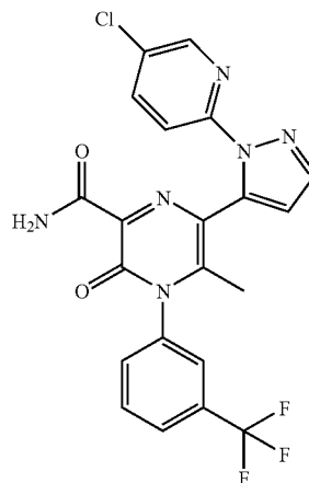
6-[1-(5-Chloropyridin-2-yl)-1H-pyrazol-5-yl]-5-methyl-3-oxo-4-[3-(trifluoromethyl)phenyl]-3,4-dihydropyrazine-2-carboxamide
