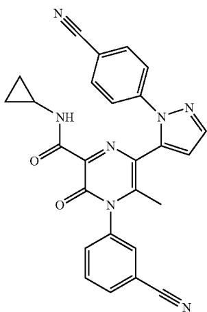
4-(3-Cyanophenyl)-6-[1-(4-cyanophenyl)-1H-pyrazol-5-yl]-N-cyclopropyl-5-methyl-3-oxo-3,4-dihydropyrazine-2-carboxamide
