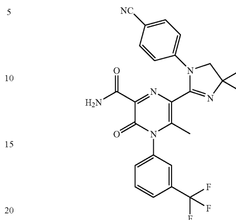
6-(1-(4-Cyanophenyl)-4,4-dimethyl-4,5-dihydro-1H-imidazol-2-yl)-5-methyl-3-oxo-4-(3-(trifluoromethyl)phenyl)-3,4-dihydropyrazine-2-carboxamide
