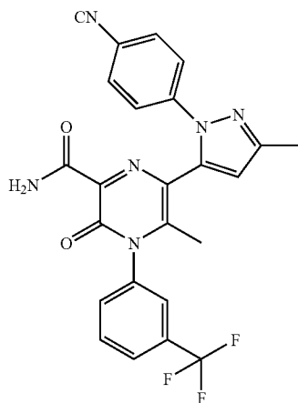
6-[1-(4-Cyanophenyl)-3-methyl-1H-pyrazol-5-yl]-5-methyl-3-oxo-4-[3-(trifluoromethyl)phenyl]-3,4-dihydropyrazine-2-carboxamide
