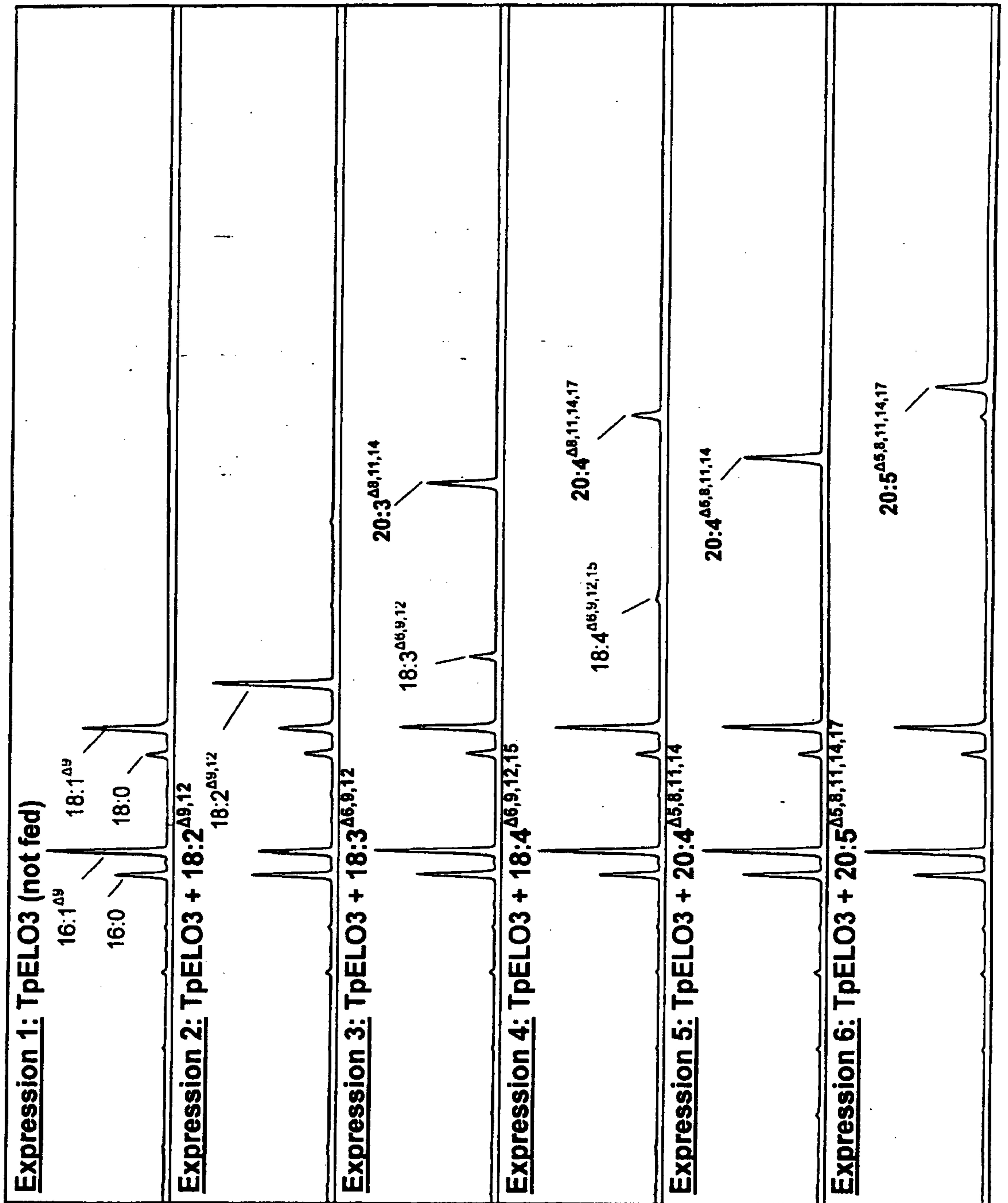
Figure 10: Expression of TpELO3 in yeast
