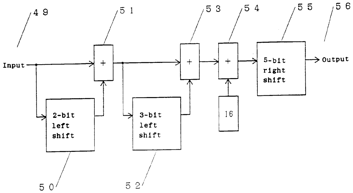
Fig. 12 Multiplier 48
