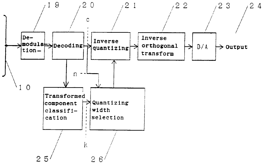
Fig. 9 Quantizing part 5
