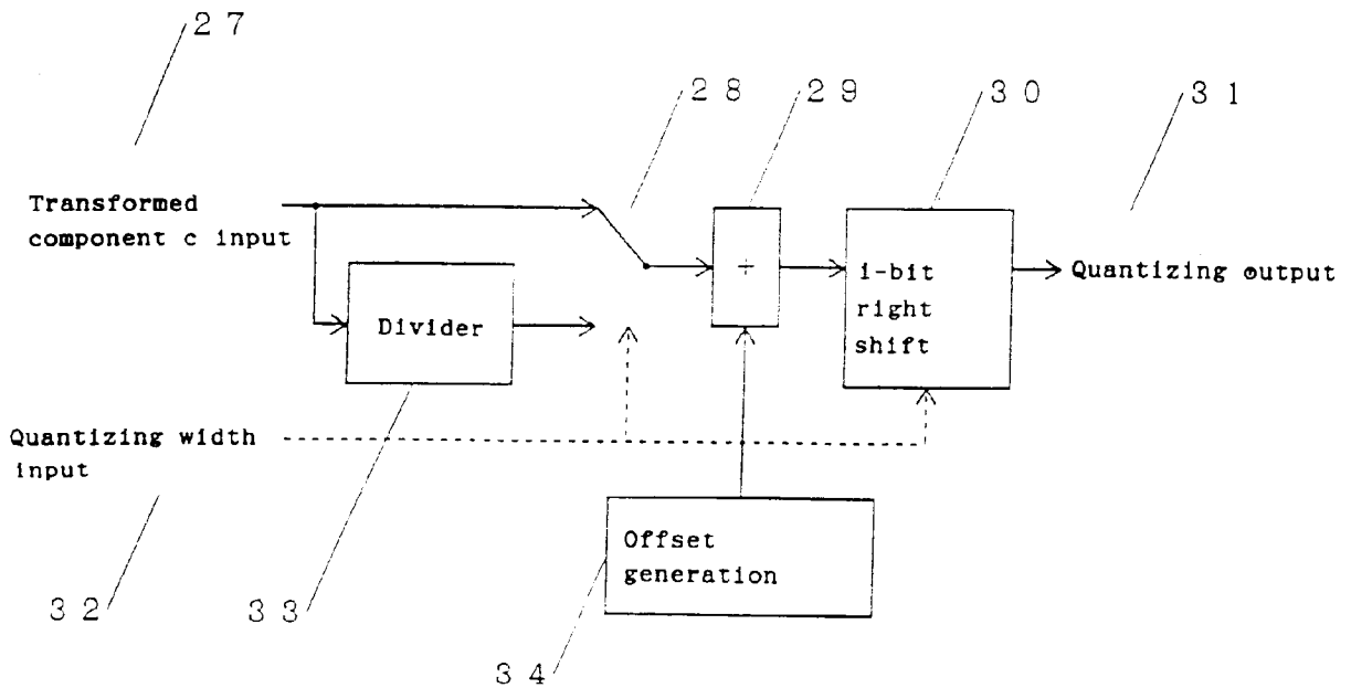
Fig. 9 Quantizing part 5
