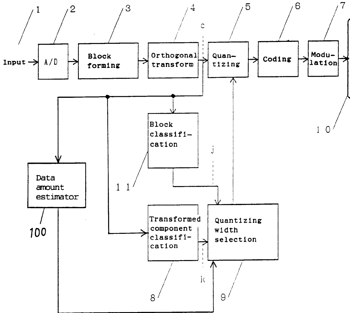
Fig. 5 Block classification 11
