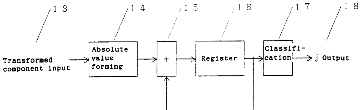
Fig. 5 Block classification 11
