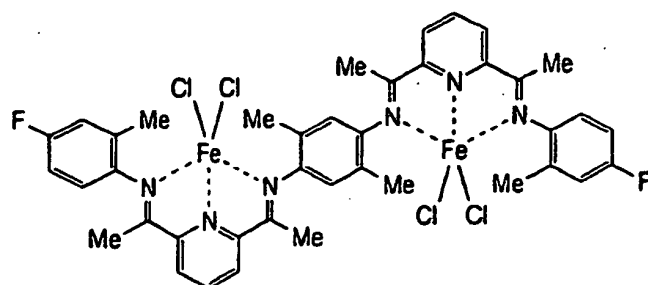
[ COMPOUND 10 ]
