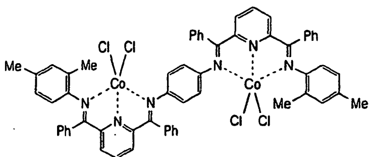
[ COMPOUND 44 ]
