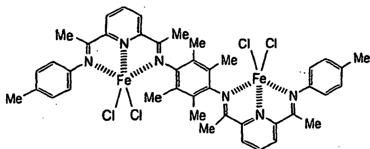
[ COMPOUND 28 ]
