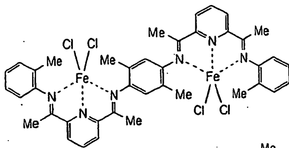
[ COMPOUND 1 ]
