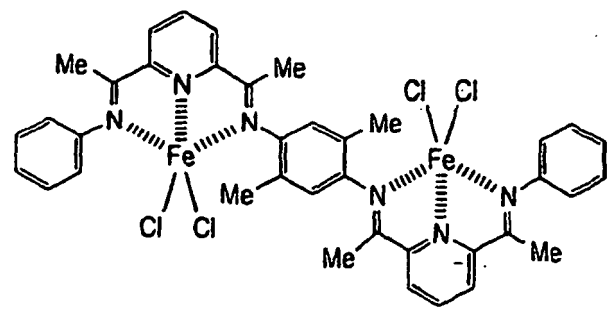
[ COMPOUND 31 ]
