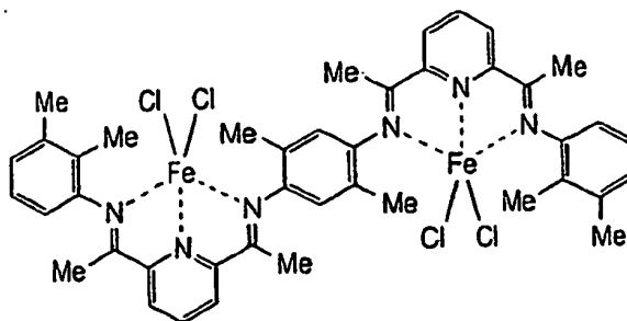
[ COMPOUND 2 ]
