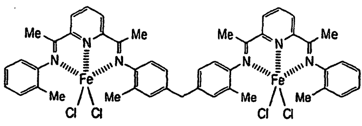
[ COMPOUND 30 ]
