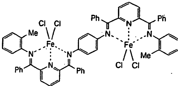
[ COMPOUND 36 ]
