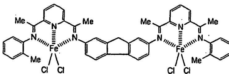
[ COMPOUND 46 ]
