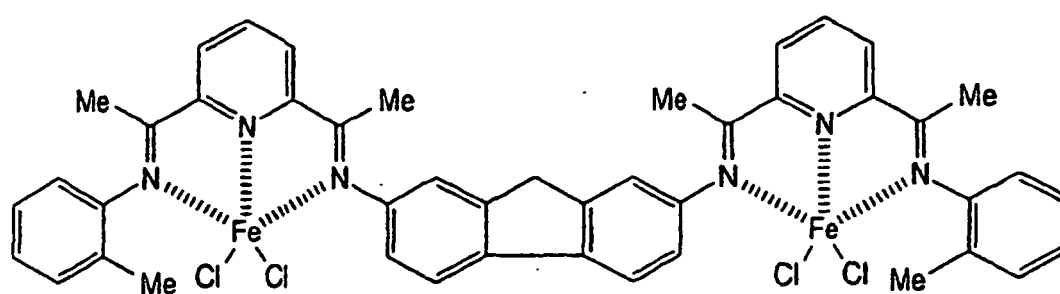
(COMPOUND 46)
