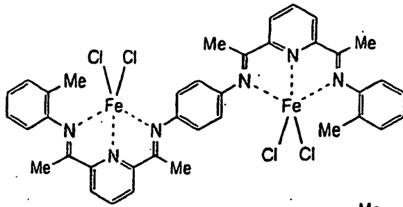
[ COMPOUND 32 ]
