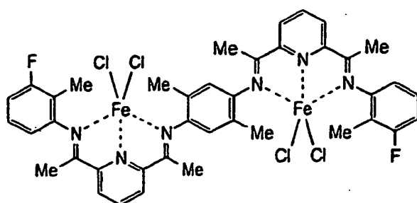
[ COMPOUND 9 ]
