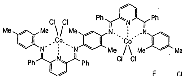
[ COMPOUND 13 ]
