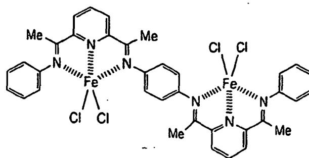
[ COMPOUND 47 ]
