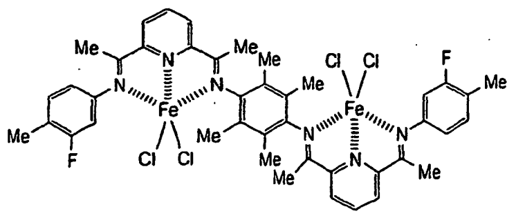
[ COMPOUND 29 ]
