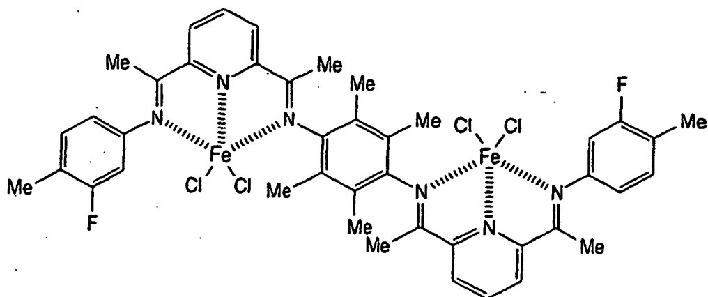
(COMPOUND 29)
