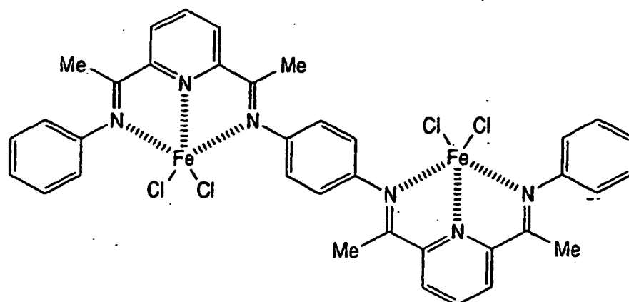
(COMPOUND 47)
