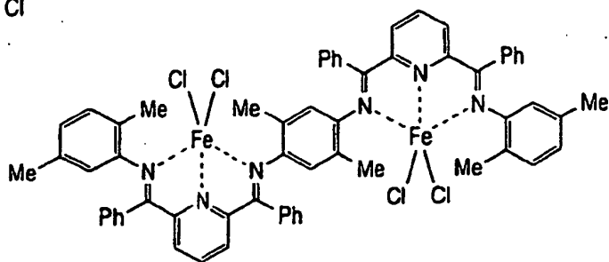
[ COMPOUND 8 ]
