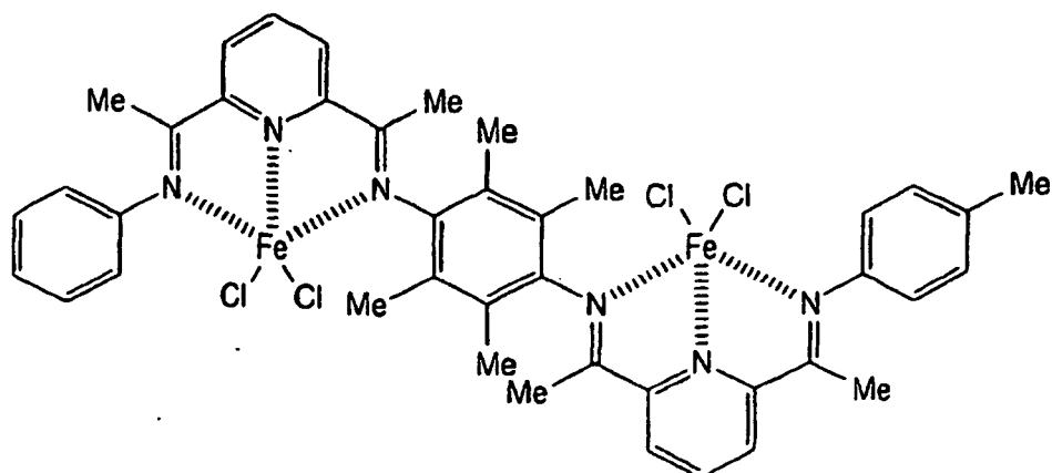
(COMPOUND 28)
