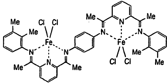
[ COMPOUND 33 ]
