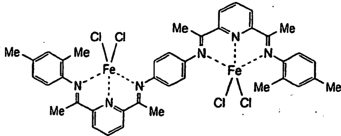
[ COMPOUND 34 ]
