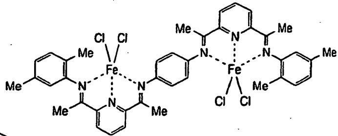
[ COMPOUND 35 ]
