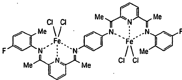
[ COMPOUND 42 ]
