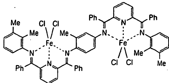
[ COMPOUND 37 ]
