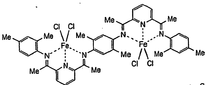
[ COMPOUND 3 ]
