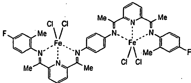
[ COMPOUND 41 ]
