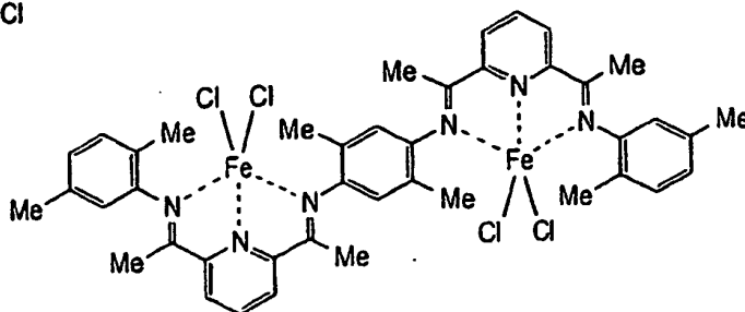
[ COMPOUND 4 ]
