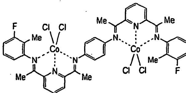
[ COMPOUND 45 ]
