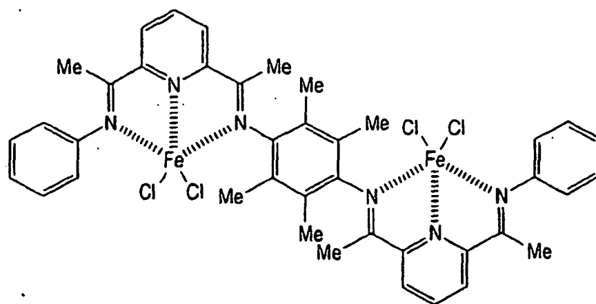
(COMPOUND 31)
