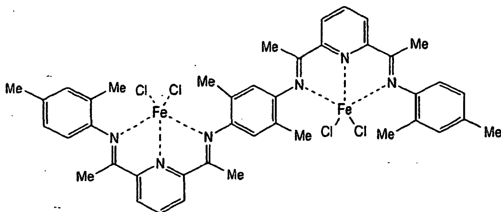
(COMPOUND 3)
