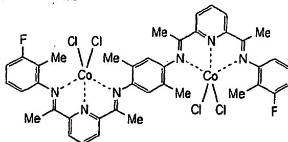
[ COMPOUND 14 ]
