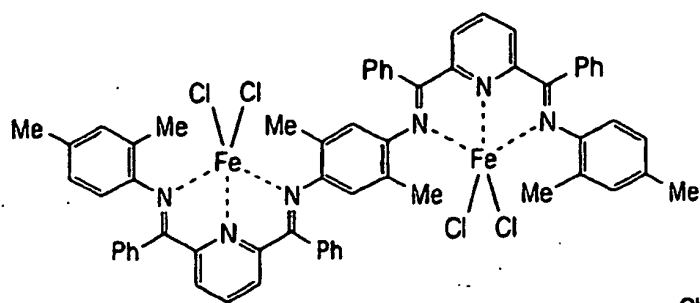
[ COMPOUND 7 ]
