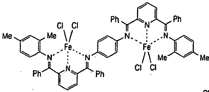
[ COMPOUND 38 ]
