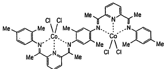
[ COMPOUND 12 ]
