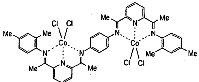
[ COMPOUND 43 ]
