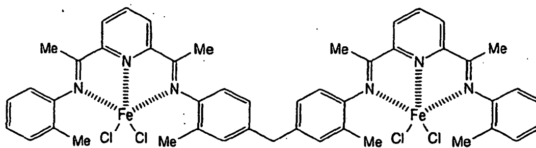
(COMPOUND 30)
