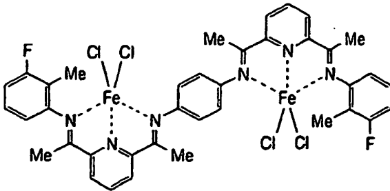
[ COMPOUND 40 ]
