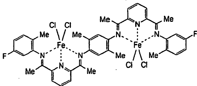
[ COMPOUND 11 ]
