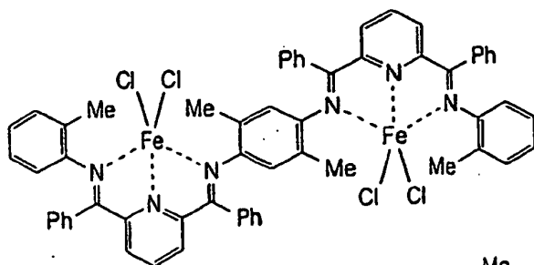
[ COMPOUND 5 ]
