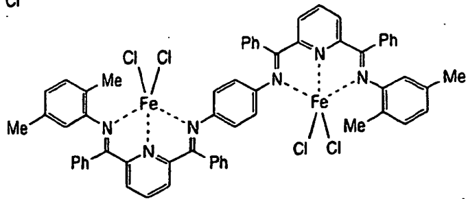
[ COMPOUND 39 ]
