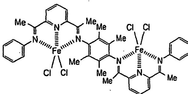
[ COMPOUND 27 ]
