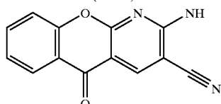
2-amino-3-cyano-azaxanthone (2ACAX)
