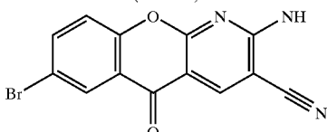
2-amino-3-cyano-azaxanthone (2ACAX)
