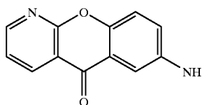
7-amino-1-azaxanth-5-one (7AAX)
