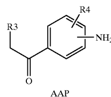
AAP
