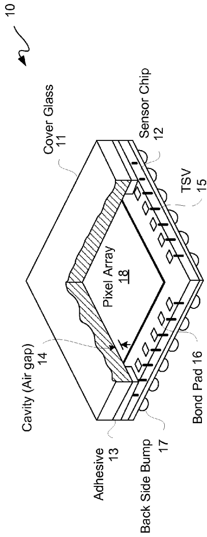
FIG. 1 (PRIOR ART)
