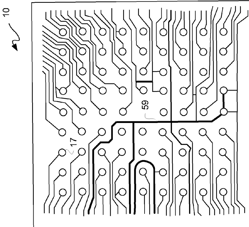
FIG. 6 (Prior Art)
