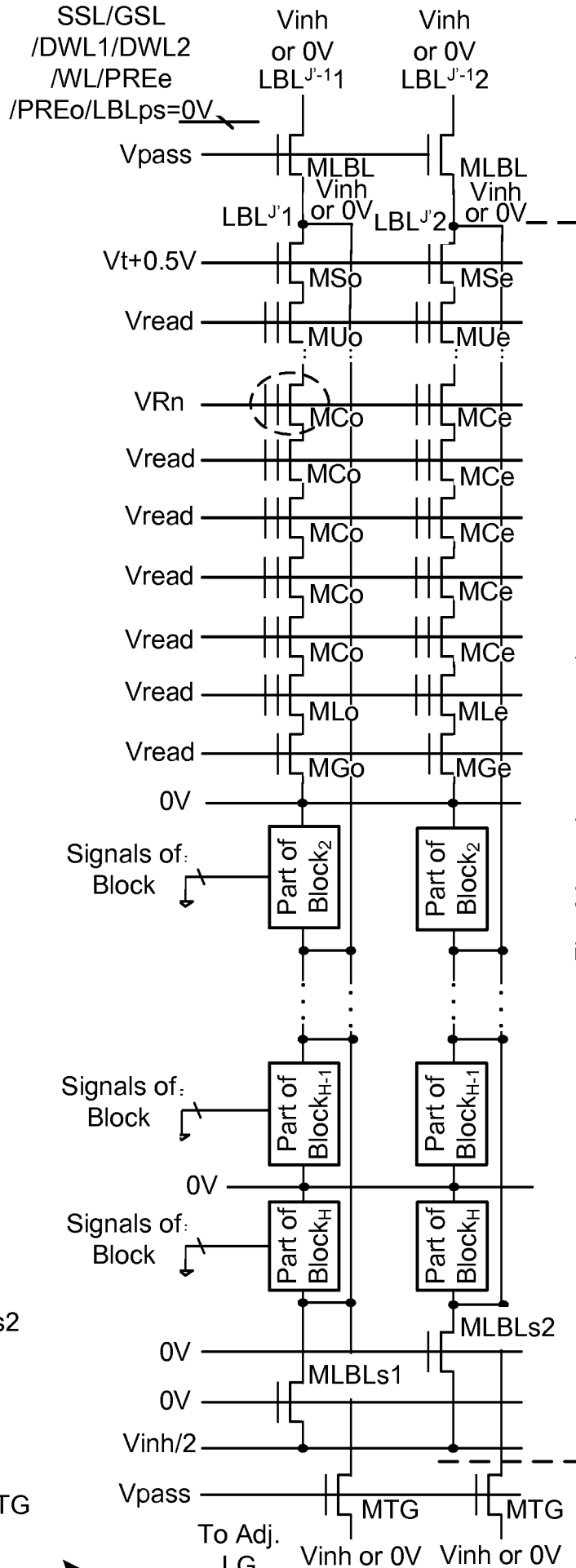
Concurrent Discharge C_{L_{BL1}} = C_{L_{BL2}} = 0V when selected V_t < V_{Rn}
