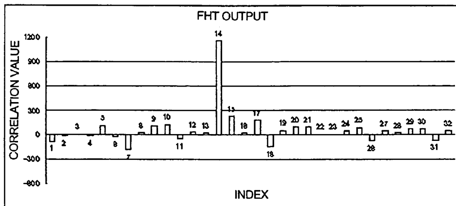
CORRELATION VALUE AFTER HADAMARD TRANSFORM
