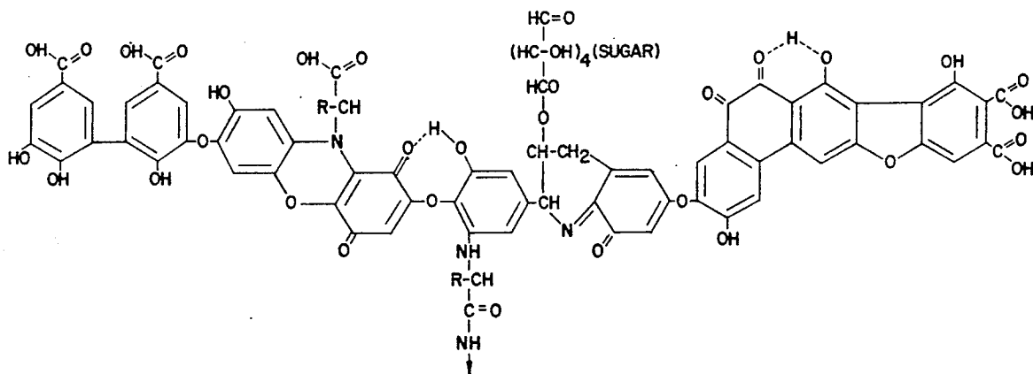
THEORETICAL STRUCTURE OF HUMIC ACID
