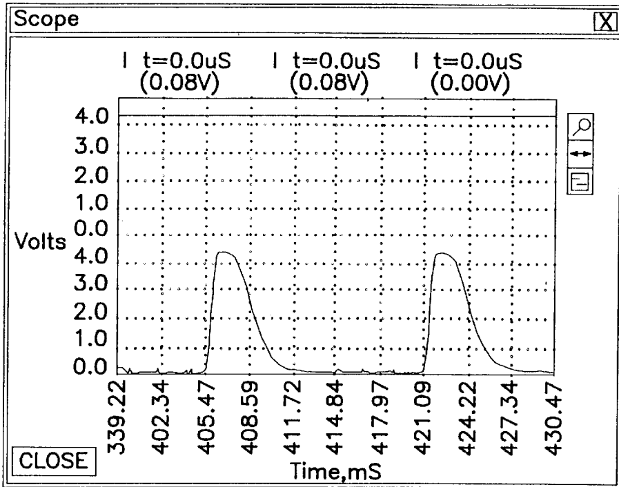
CRT photoresponse
