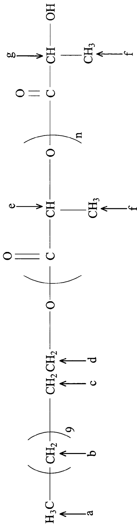
Mono-functional PLLA
