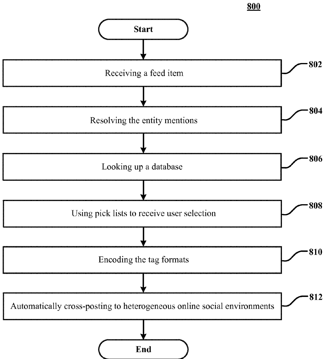
FIG. 8 – Flow Chart of Entity Mentions Conversion
