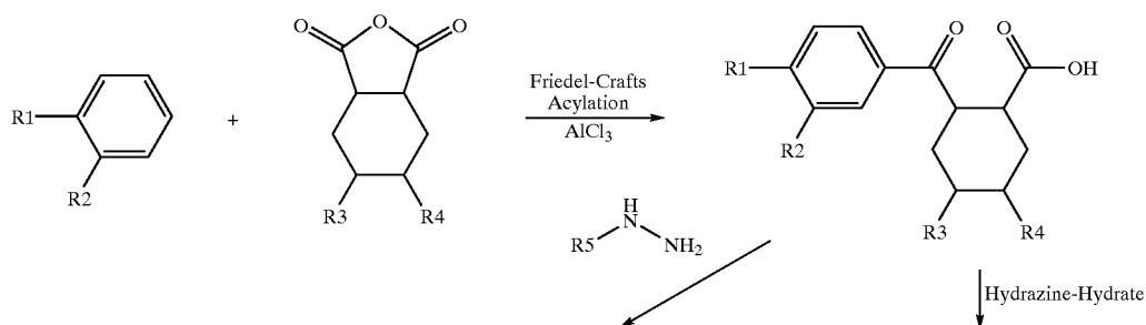
Reaction scheme 1:
