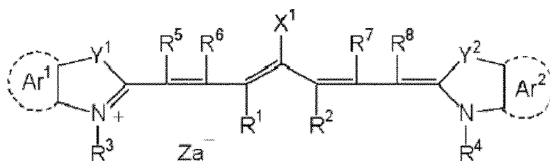
Formula (a)
